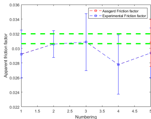
Figure: Comparison between Experimental Friction factor and Aasgard Friction Factor
