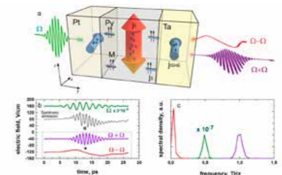
Spintronics THz second harmonic generation and optical rectification in ferromagnet-heavy metal trilayers.
