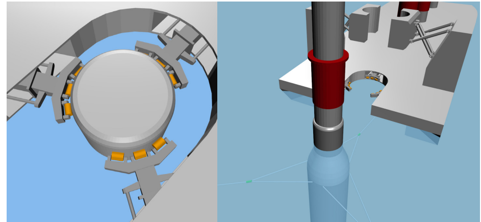
Figure 6. Illustrations of the gripper design and the lifting mechanism.
