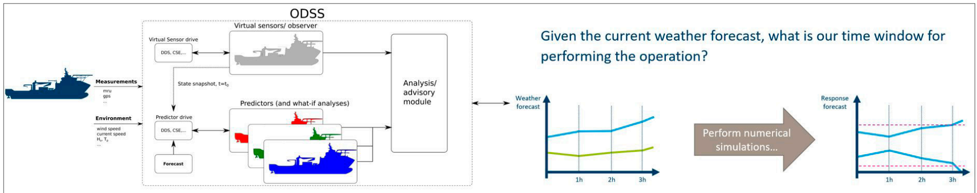
Figure 14. Main components and interfaces in an ODSS architecture.
