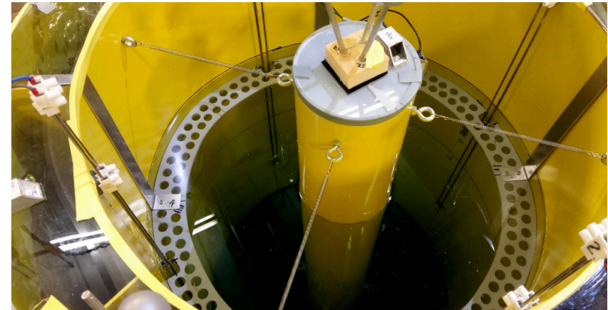
Figure 12. Floating dock with the spar of a Hywind wind turbine inside
